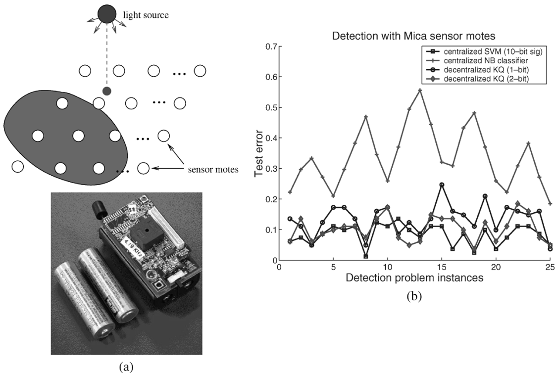
Fig. 4. (a) Sensor field (top) and a Mica sensor mote (bottom). (b) Comparison of test errors of the decentralized KQ algorithm and centralized SVM and NBC algorithms on different problem instances.
