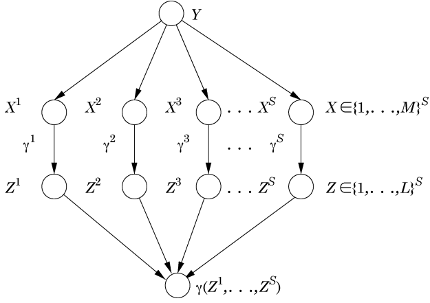
Fig. 1. Decentralized detection system with S sensors, in which Y is the unknown hypothesis X = (X^1, \dots, X^S) is the vector of sensor observations, and Z = (Z^1, \dots, Z^S) are the quantized messages transmitted from sensors to the fusion center.
